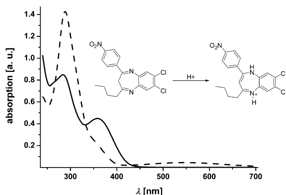
Figure 4. Absorption (recorded in \text{CH}_2\text{Cl}_2 at 293 K) spectra of 6i (solid line) and 6i-H + (dotted line).
