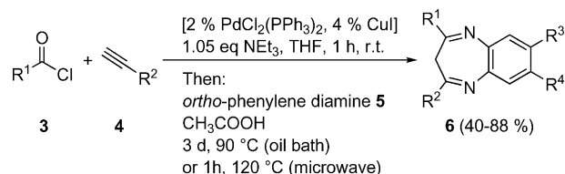
Scheme 1. One-pot three-component synthesis of 1,5-benzodiazepines 6 .
