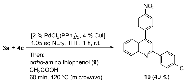
Scheme 3. One-pot three-component synthesis of quinoline 10 .
