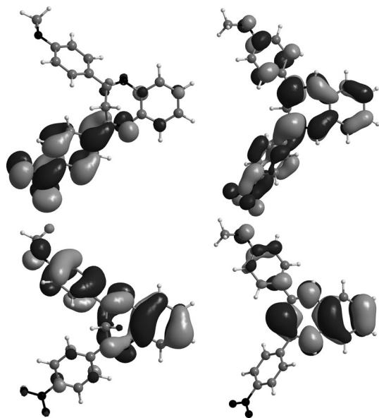
Figure 6. DFT-computed frontier orbitals of 1,5-benzodiazepines 6n (left) and 6n-H + (right), LUMOs (top) and HOMOs (bottom).
