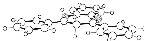
Figure 3. Optimized transition state of the 2,4-diphenyl-substituted 1,5-benzodiazepine.
