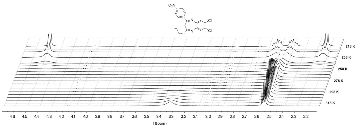
Figure 2. Temperature-dependent 1 H NMR spectra of compound 6j , selected signals (recorded in CDCl 3 , 500 MHz).
