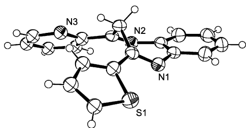
Figure 1. Molecular structure of compound 6f .
